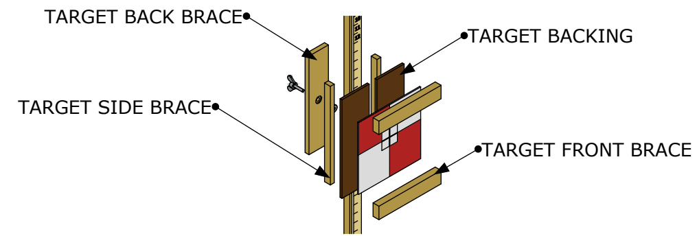
TARGET EXPLODED VIEW
